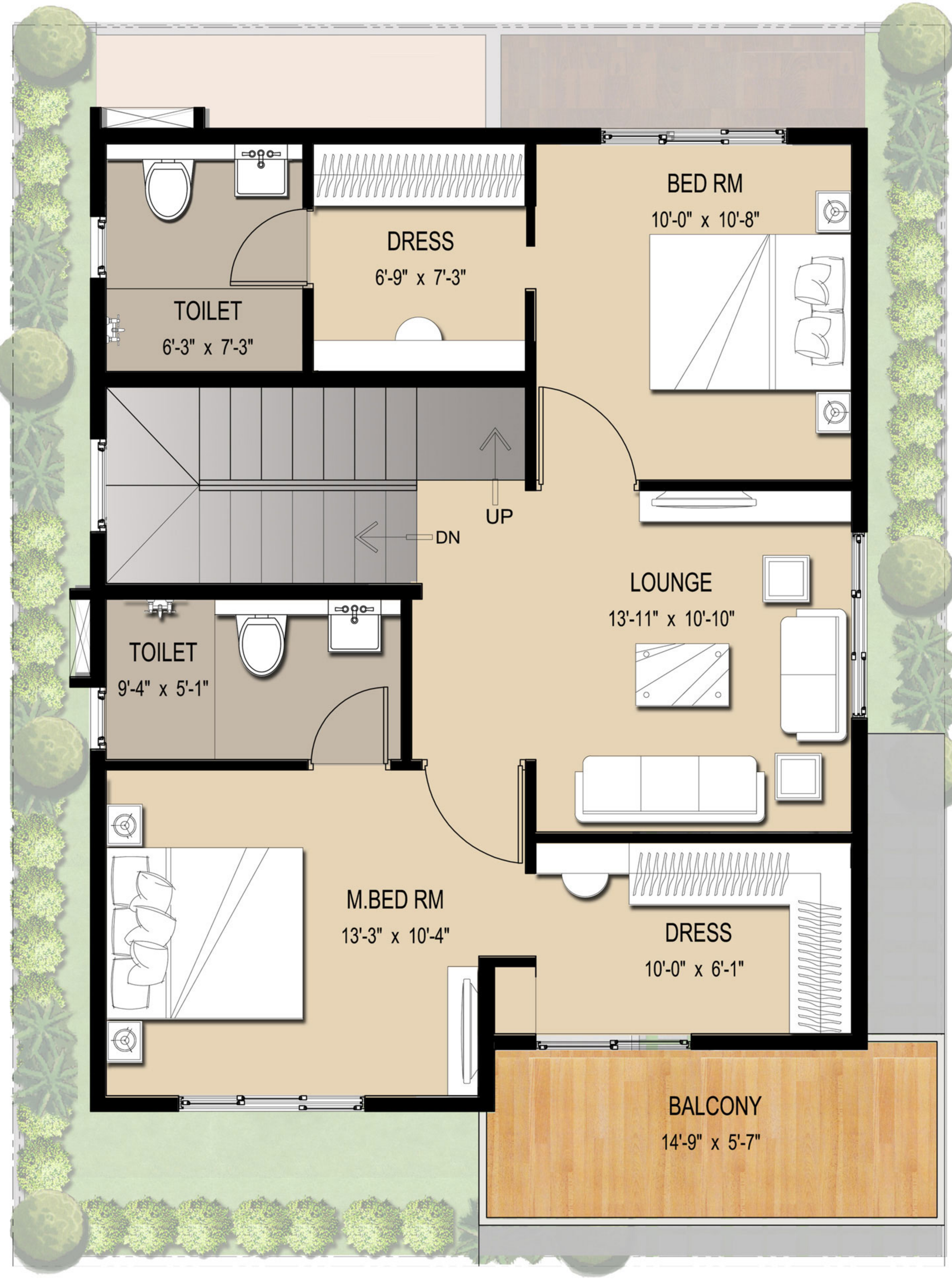
FIRST FLOOR
